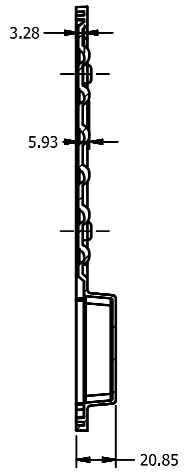
SECTION E-E
