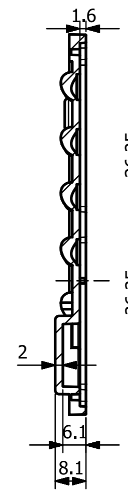
SECTION H-H
