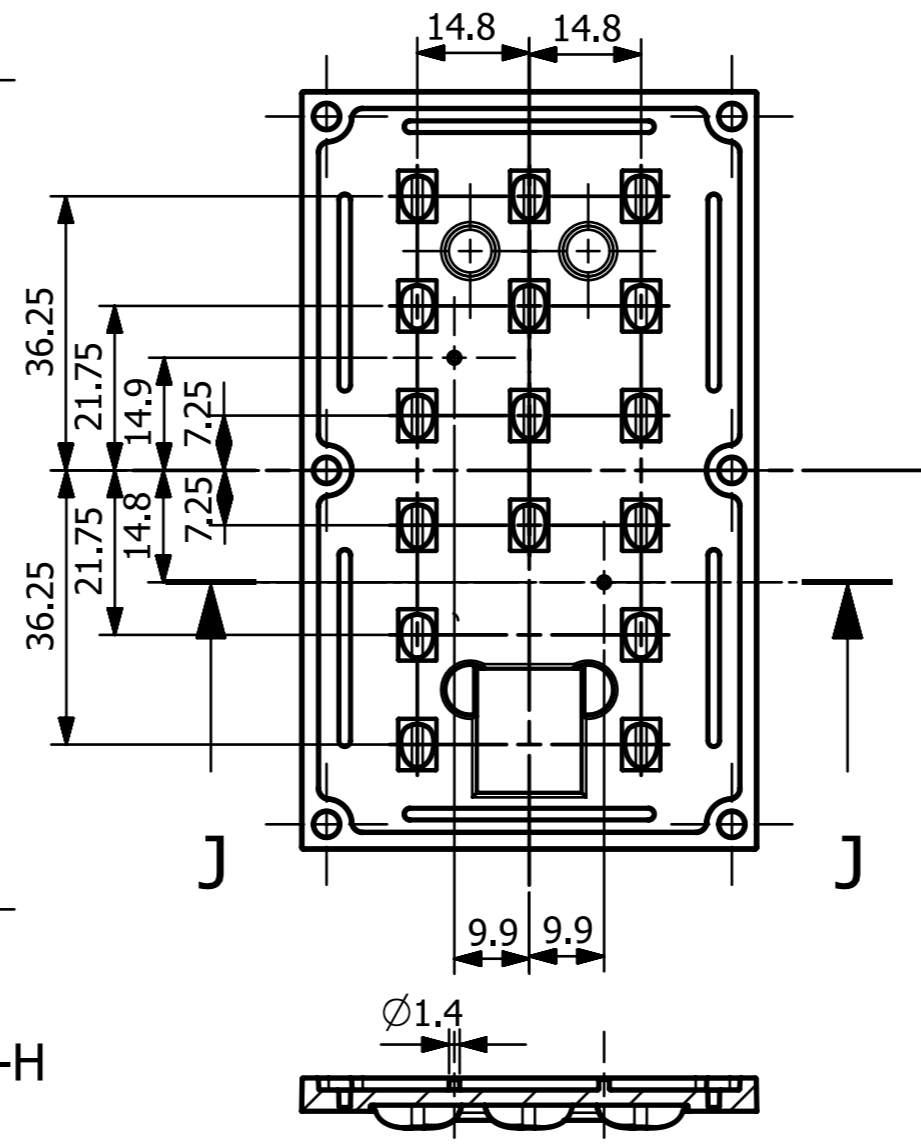
SECTION J-J
