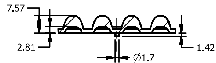
SECTION E-E
